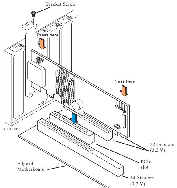
Figure 2 Installing the MegaRAID SAS 9280-8e/9280DE-8e RAID Controller
