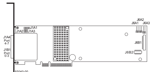
Figure 1 Layout of the MegaRAID SAS 9280-8e/9280DE-8e RAID Controller
