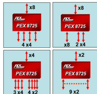
Figure 1. Single-Host Port Configurations
