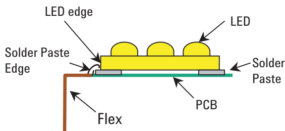
Figure 1. Rigid flex assembly.
