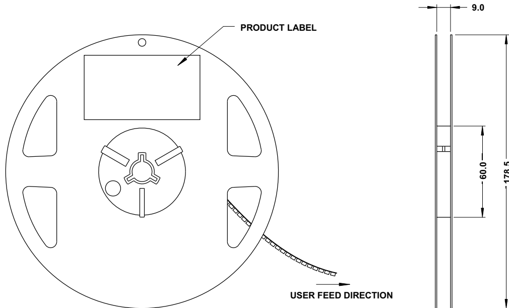
Figure 21: Reel Dimensions
