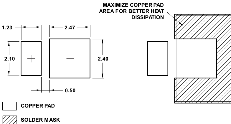
Figure 19: Recommended Soldering Land Pattern
