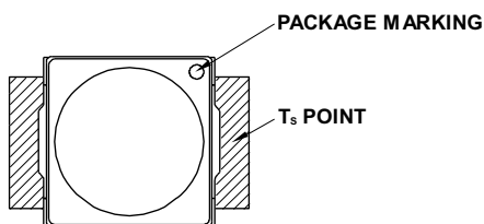
Figure 23: Solder Point Temperature on PCB
