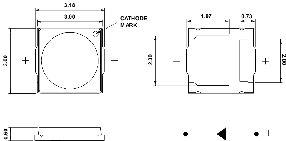
Figure 1: Package Drawing
