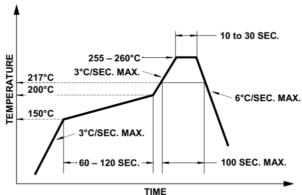
Figure 22: Recommended Lead-Free Reflow Soldering Profile
