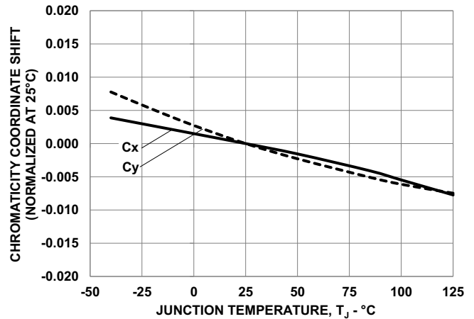
Figure 14: Chromaticity Coordinate Shift vs. Junction Temperature – 4000K
