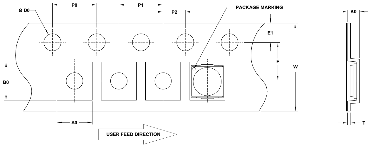
Figure 20: Carrier Tape Dimensions
